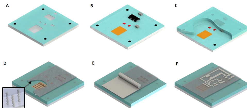
Figure 2. Fabrication process with UVLM. (A) PDMS substrate is applied onto a glass plate. Placement openings and fiducials are patterned with UV laser for placing surface mount components and laser alignment, respectively. (B) Surface mount electronic components are placed into the openings with PVA as a bonding agent. (C) The components are then sealed in PDMS. (D) The chip-embedded elastomer is peeled from the glass plate, flipped over, and coated with a layer of zPDMS. (E) A film of EGaIn is applied on the zPDMS with a PDMS roller and then (F) patterned with a UVLM system. Lastly, the LM circuit is sealed in PDMS and released from the glass substrate.
