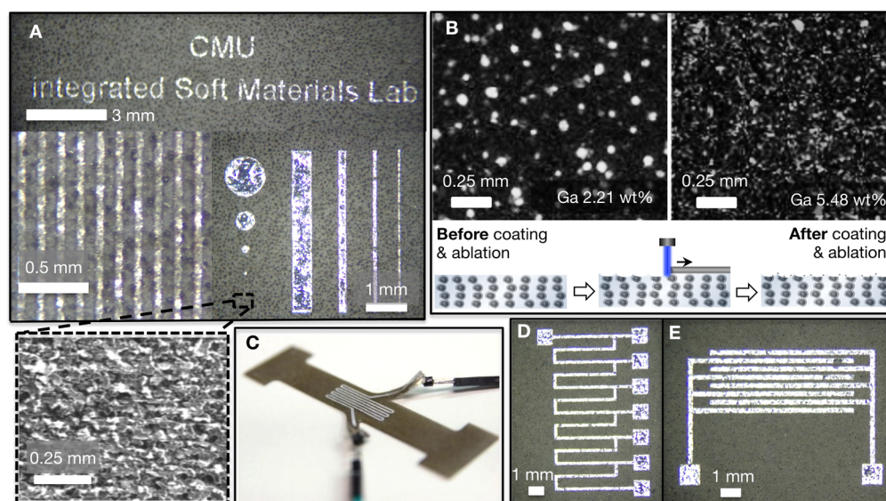
Figure 3. Samples of UV laser-patterned EGaIn features. (A) The planar dimensions of patterned traces can be as small as 50\ \mu\text{m} . The SEM image in the inset shows the rough surface of zPDMS after laser ablation. (B) The EDS image of elemental distribution of Ga before and after EGaIn coating and laser ablation. (C) Serpentine circuit used to measure electrical resistance during stretch. (D) EGaIn circuit with multiple terminals for measuring the influence of trace length on resistance. (E) Interdigitated capacitor for measuring trace length on capacitance.
