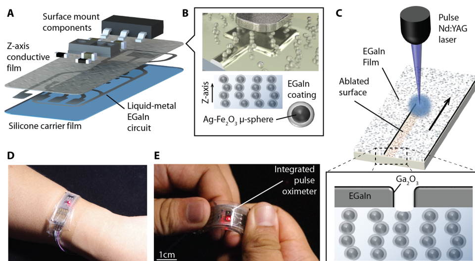
Figure 1. Liquid–metal soft-matter electronics. (A) Illustration of soft-matter bioelectronic skin. (B) Vertically aligned columns of Ag–Fe 2 O 3 microparticles coated in EGaIn act as z-axis interconnects between LM trace terminals and surface-mounted components. (C) Illustration of EGaIn patterned using UVLM. During patterning within an oxygen-rich environment, the growth of Ga 2 O 3 is necessary to hold the shape of the LM circuit (see inset). (D) Soft-matter bioelectronic skin with integrated pulse oximeter that can be worn as a wrist band and (E) support mechanical deformation during operation.
