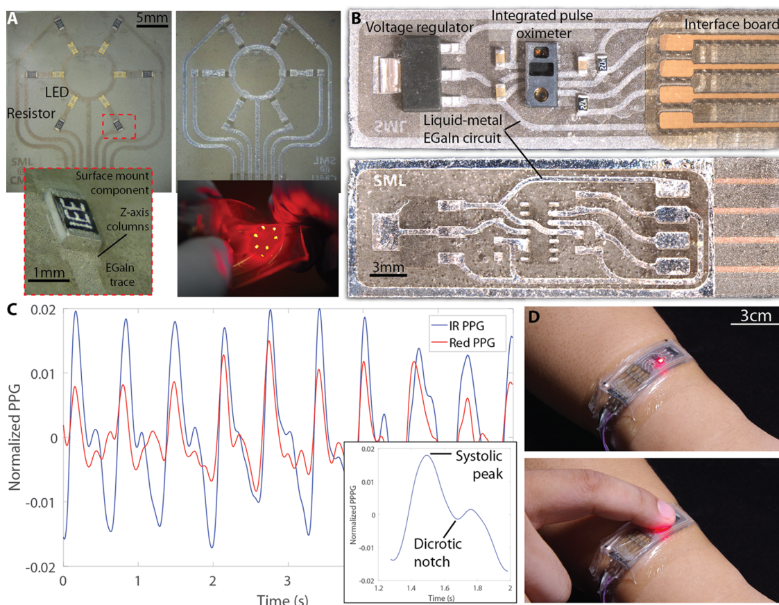
Figure 5. Soft-matter printed circuit board implementation. (A) Top and bottom of a circuit containing a circular array of LEDs. Inset, bottom left: close up of interface between resistor and EGaIn trace; inset, bottom right: soft-matter LED array undergoing deformation during operation. (B) Top and bottom of soft-matter pulse oximeter circuit. (C) PPG waveform recorded from soft-matter pulse oximeter shown in (B); (C) inset: magnified view of single cardiac beat from the measured PPG waveform. (D) Possible implementation of soft-matter pulse oximeter worn as wristband. PPG waveform can be recorded by placing finger on top of wristband while applying light pressure.
