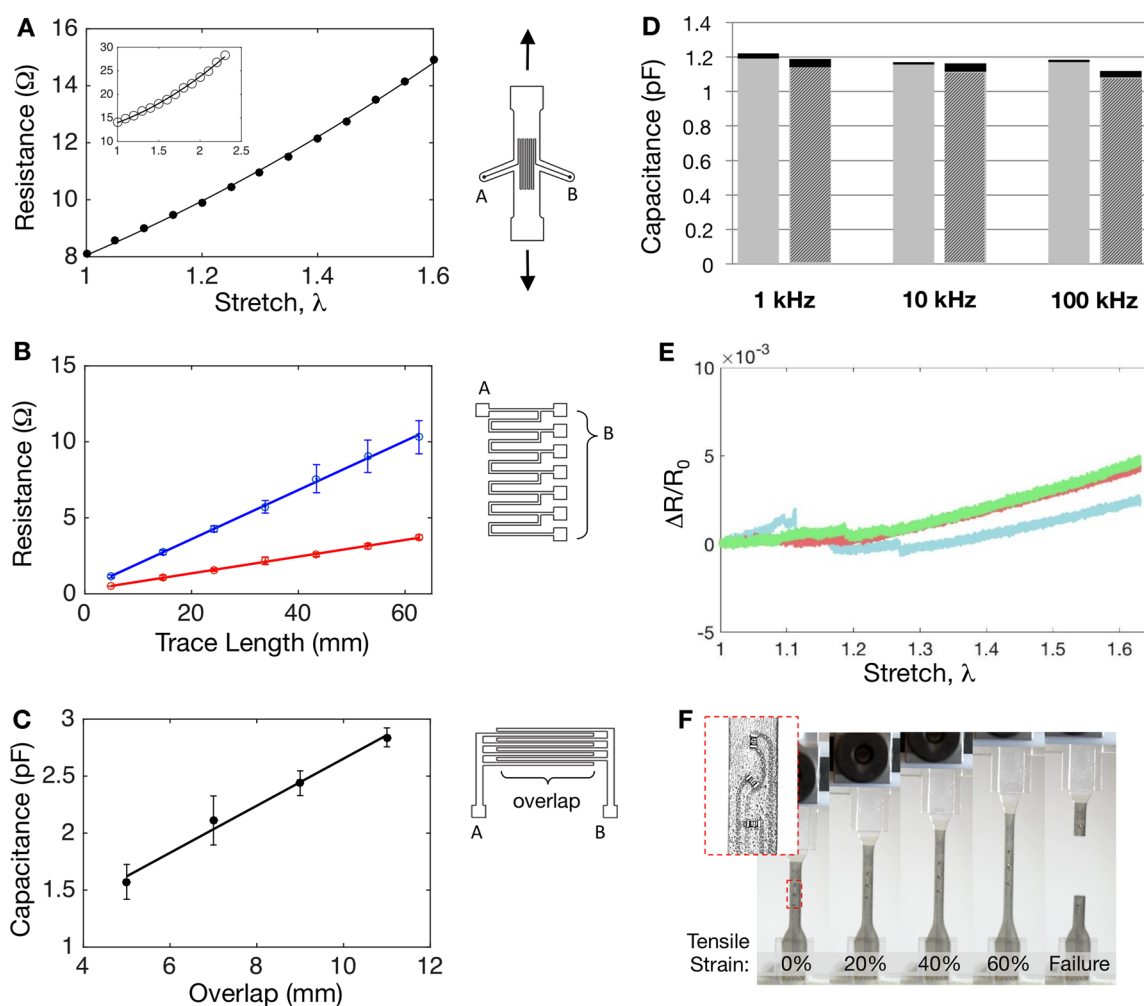
Figure 4. UVLM patterned planar resistors and capacitors. (A) Experimental measurements (markers) and theoretical fit (curve) for electrical resistance versus stretch for serpentine LM trace (120 mm length, 0.5 mm width); Inset: measurement of laser-patterned LM trace encapsulated between two layers of soft polyacrylate elastomer (VHB Tape 4910; 3M). (B) Resistance versus trace length for 100 \mu\text{m} (red) and 200 \mu\text{m} wide (blue) traces. Markers and curves correspond to experimental measurements and theoretical fit, respectively. (C) Experimental measurements (markers) and theoretical fit (curve) for capacitance versus overlap length of interdigitated LM traces (250 \mu\text{m} width, 150 \mu\text{m} spacing). (D) Average capacitance of comb capacitors patterned with (gray) UVLM and (hatched gray) stencil lithography for various testing frequencies. The black bars are the standard deviation ( N = 9 ). (E) Plot of change in electrical resistance versus stretch for surface mount resistors oriented at 0^\circ (blue), 45^\circ (red), and 90^\circ (green). (F) Photographs of sample when strained (0, 20, 40, and 60%) and after failure. Inset: Close up of sample showing placement of resistors. All circuits were patterned on zPDMS unless otherwise noted.
