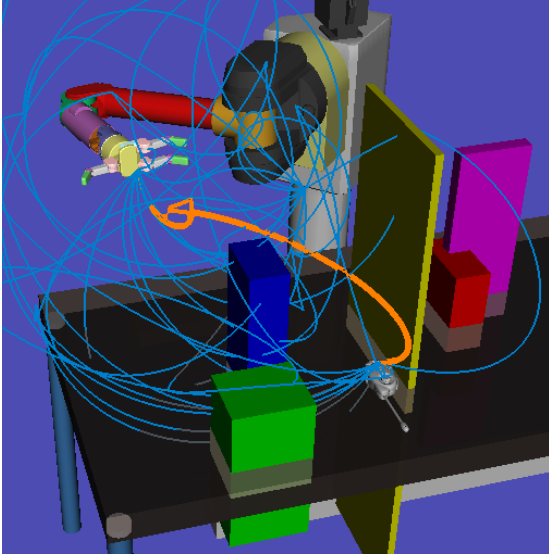
(b) The initialization seed for CHOMP found using CONSEQOPT is marked in orange. Using this initial seed CHOMP is able to find a collision free path that also has a relatively short execution time.
