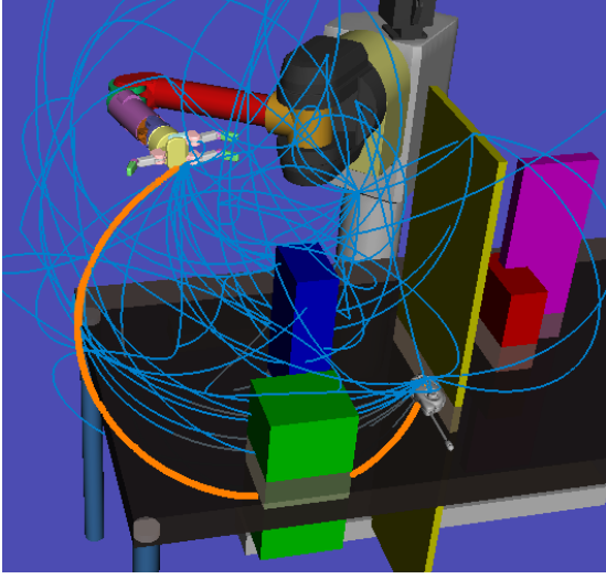
(a) The default straight-line initialization of CHOMP is marked in orange. Notice this initial seed goes straight through the obstacle and causes CHOMP to fail to find a collision-free trajectory.
