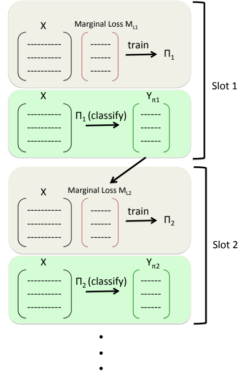
Fig. 1: Schematic of training a sequence of classifiers for regret reduction of contextual sequence optimization to multi-class, cost-sensitive, classification. Each slot has a dedicated classifier which is responsible for predicting the action with the maximum marginal benefit for that slot.
