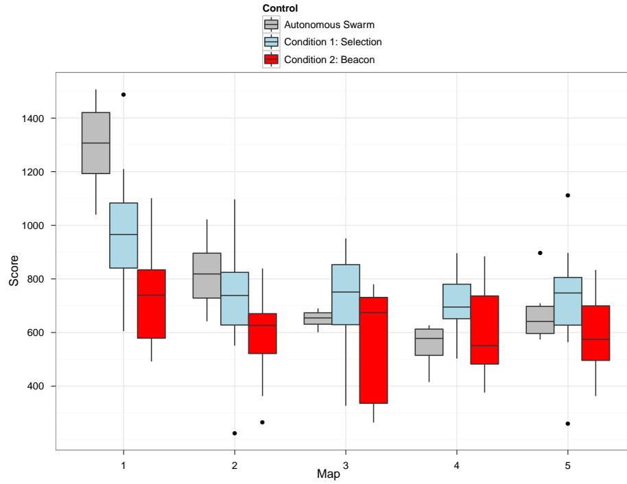
Figure 6. A box plot of the scores across participants for maps 1 to 5. Note that these scores only include missions with 100 robots and participants have either only map 3 or only map 4 with 100 robots, i.e. the sample size is reduced for map 3 and 4.
