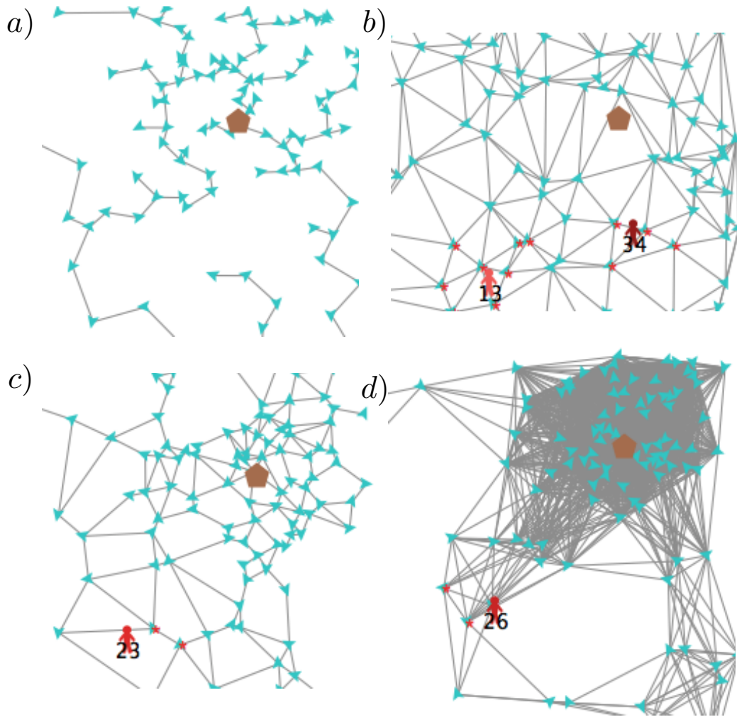
Figure 4. An illustration of the communication graphs with connections as straight grey lines between robots: a) minimum spanning tree, b) Delaunay graph, c) r_c -limited Gabriel graph, and d) r_c -disk graph.
