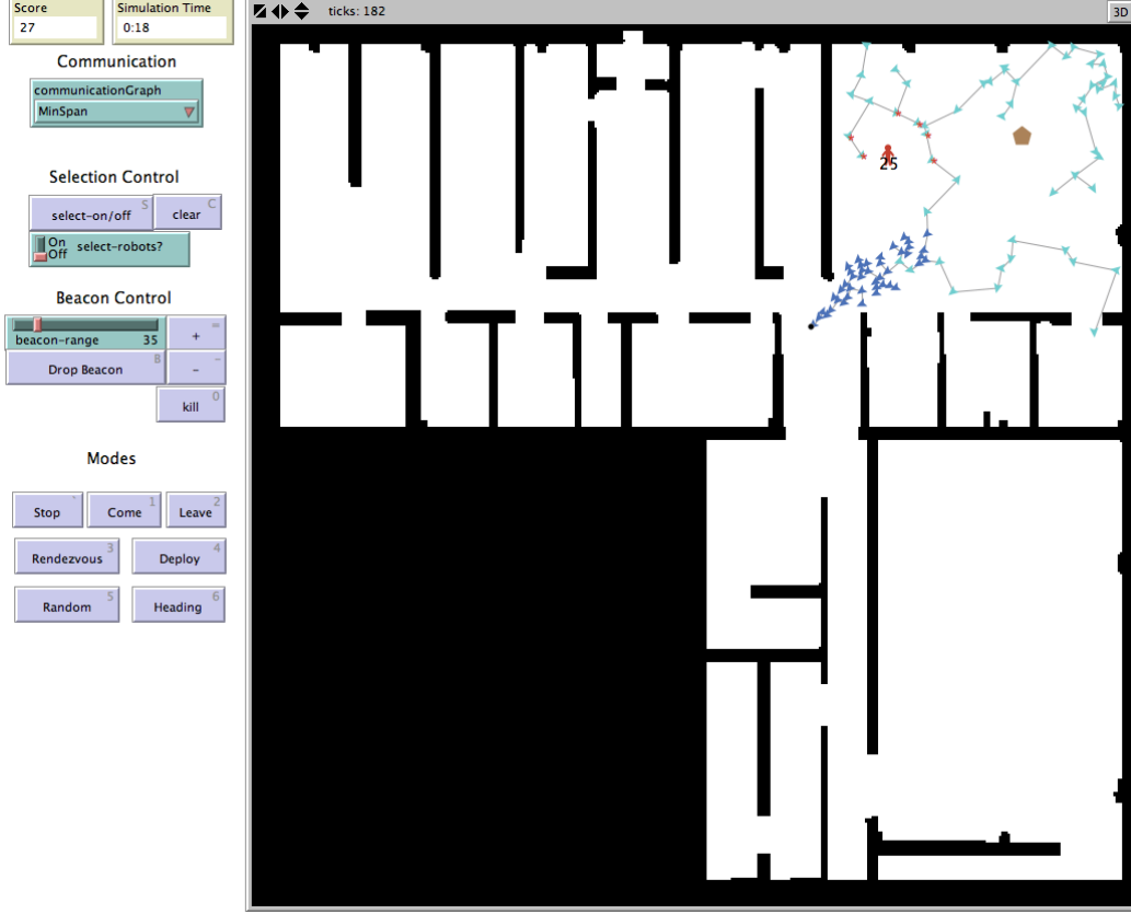
Figure 3. The user interface of the swarm testbed. Robots are small arrows, communication links are grey edges, the base station is brown, and information objects are marked as persons (information objects) in red with their information value displayed in black. Robots currently within information range r_i of an information object receive a red “*”. Operators in the beacon and in the selection control conditions only see their respective control panel.
