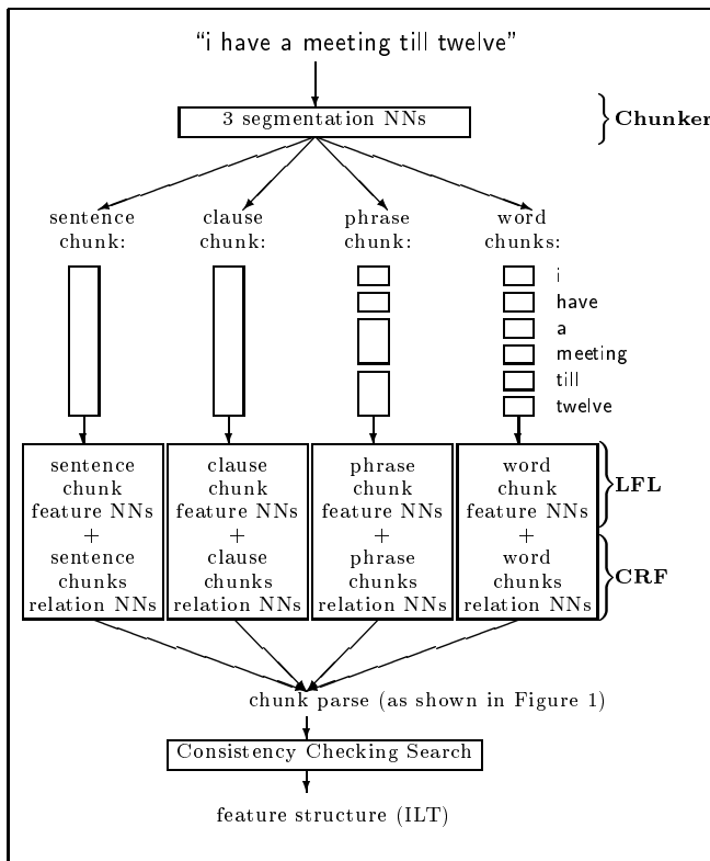
Figure 2: FeasPar’s architecture for run mode.
