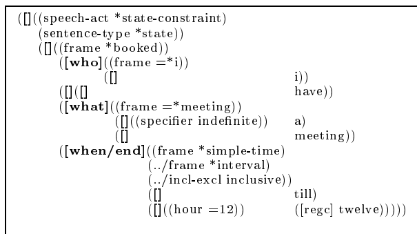
Figure 1: Chunk parse (chunk relations shown in boldface)
