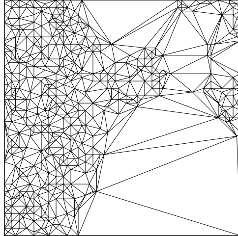
Figure 2: A triangulation \mathcal{T}S using 512 vertices that approximates H ; an example of a triangulated irregular network.
