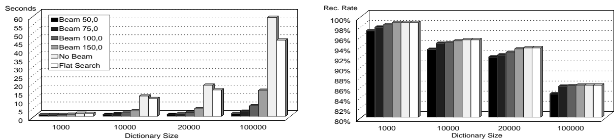
Figure 3: Recognition times (left) and recognition results (right) for different beam sizes and dictionary sizes from 1,000 words up to 100,000 words.
