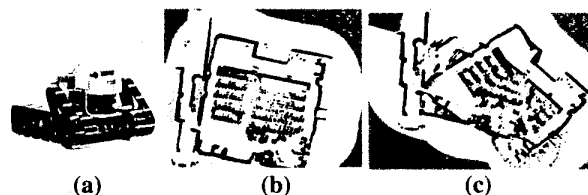
Figure 1 Typical example of global mapping using a single-scan laser range finder; (a) SICK laser mounted on a mobile platform; (b) final map of building; (c) initial map from odometry only (from Thrun.)
