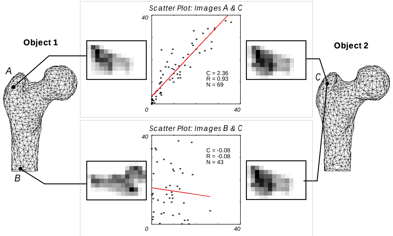
Figure 5: Comparison of spin-images visualized as scatter plots.
