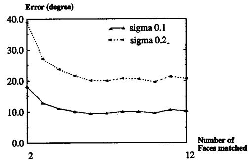
Fig. 8. Reconstructed error vs. number of matched faces.
