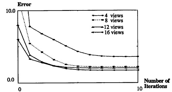
Fig. 7. Effect of number of views.
