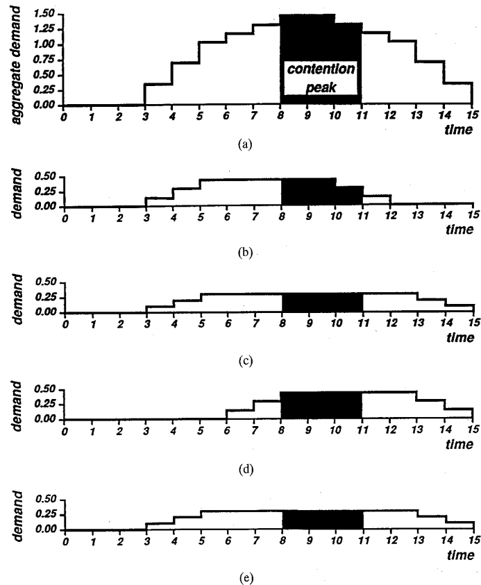
Fig. 6. Activity ordering by agent \alpha and \beta . (a) Aggregate demand for resource R_2 . (b) Activity A_2^\alpha 's demand for R_2 . (c) Activity A_3^\beta 's demand for R_2 . (d) Activity A_3^\beta 's demand for R_2 . (e) Activity A_2^\beta 's demand for R_2 .
