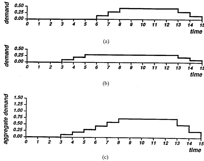
Fig. 3. Building agent \beta 's demand for resource R_2 . (a) Activity A_2^{1,\beta} 's demand for R_2 . (b) Activity A_2^{2,\beta} 's demand for R_2 . (c) Agent \beta 's demand for R_2 .
