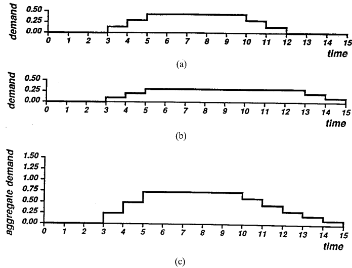
Fig. 2. Building agent \alpha 's demand for resource R_2 . (a) Activity A_2^{1,\alpha} 's demand for R_2 . (b) Activity A_2^{2,\alpha} 's demand for R_2 . (c) Agent \alpha 's demand for R_2 .
