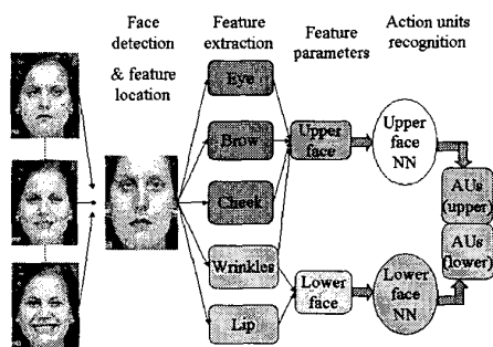
Figure 1. Feature based action unit recognition system.
