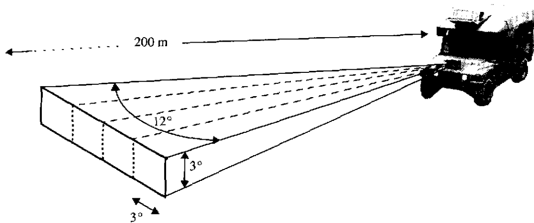
Figure 1 Sensor Geometry
