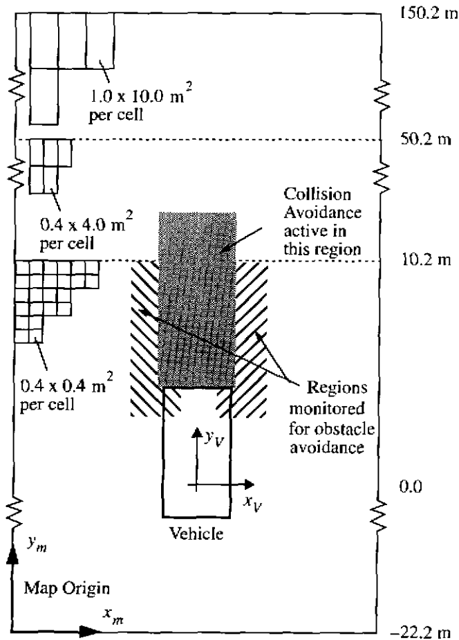
Figure 7 Local Grid Map
