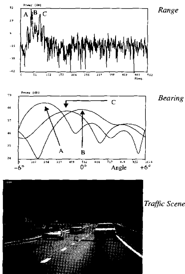
Figure 6 Radar Data obtained on Highway
