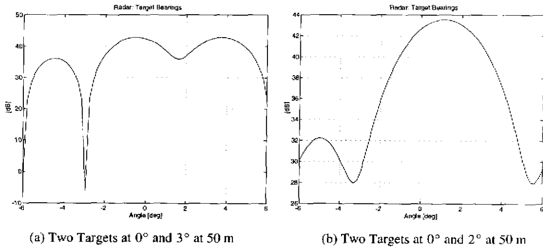
Figure 4 Resolution limit of Fourier Transform
