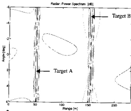
(c) Contour Plot of Range / Bearing Matrix
