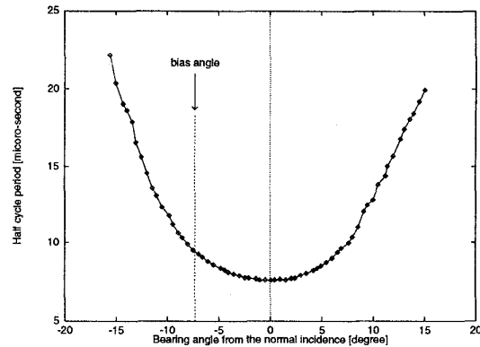
Figure 6: Relationship between angle and the half cycle period. The bias angle is used for overcoming symmetry.
