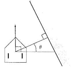
Figure 9: The perpendicular direction to the proceeding direction of the robot is set as zero degree. The measured bearing angle to the nearest point is \theta .
