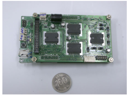
Fig. 3 Motor controller of head
